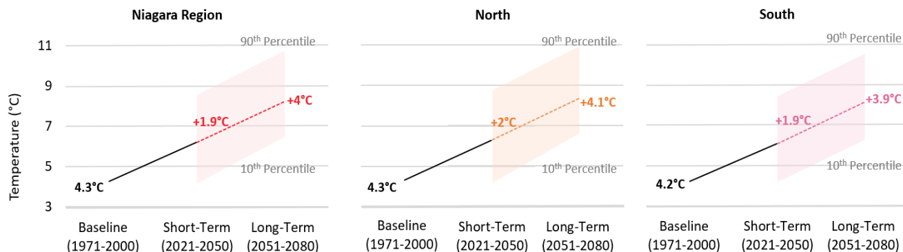
FIGURE 17: COMPARISON OF MEAN MINIMUM DAILY TEMPERATURE BETWEEN REGIONAL AND SUB-REGIONAL ANALYSIS.
